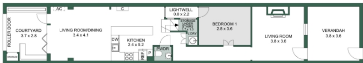
GROUND FLOOR
